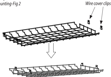
Wire guard mounting-Fig 2
