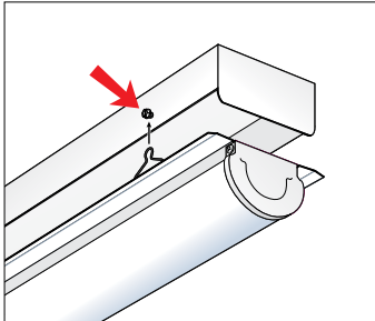
Mounting hooks easily help hang retrofit to become hands free to finish installation.
