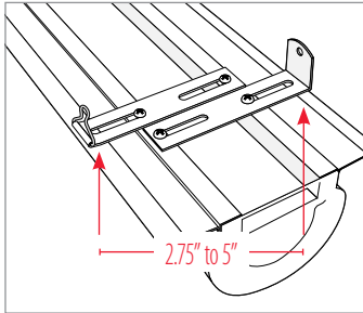
Hands are free to affix retrofit mounting brackets into place. Groove in bracket reinforces strip wall for self-tapping screw insertion.
