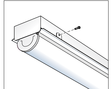
White mounting brackets attached to side of strip fixture for neat design.
